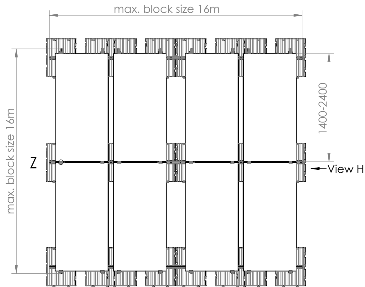
Plan view 1 : 50
